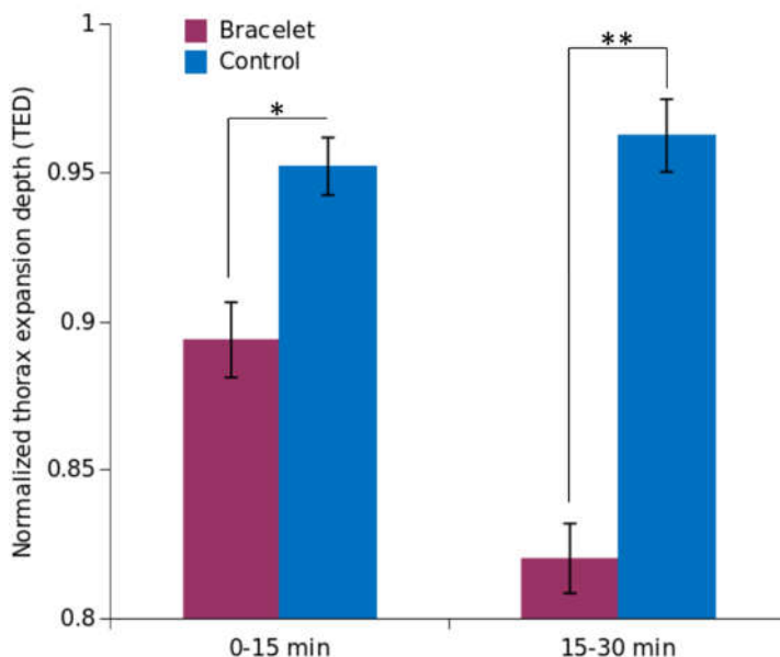
Figure 18: Normalized thorax expansion depth (TED) from fifteen volunteers during two parts of measurements for both test situations ( Bracelet : BD PROTECT EMF+ Protection Bracelet on the volunteer’s wrist, Control : sham bracelet). Mean values ± standard error (N = 15) are shown. A single asterisk (*) represents a statistically significant difference between two situations with p < 0.05 and a double asterisk (**) represents a statistically significant difference with p < 0.01 .
